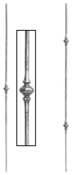
Art. 499/1 Ø 12 mm H 900 mm Art. 499/2 Ø 12 mm H 900 mm
