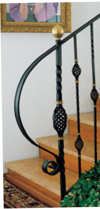
Art. 113/4/BR □ 1.1/8" H 1150 mm Art. 112/B/10/BR □ 1.1/8" H 1150 mm Art. 113/2/BR □ 1.1/8" H 1150 mm Art. 112/B/14/BR □ 1.1/8" H 1150 mm Art. 112/B/16/BR □ 1.1/8" H 1150 mm
