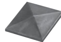
Art. 167/7 □ 80 x 80 x 2 mm H 20 mm Art. 167/8 □ 100 x 100 x 2 mm H 20 mm
